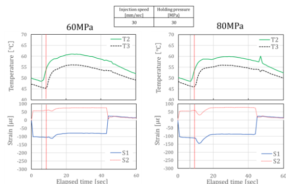
Fig. 6 Injection pressure
