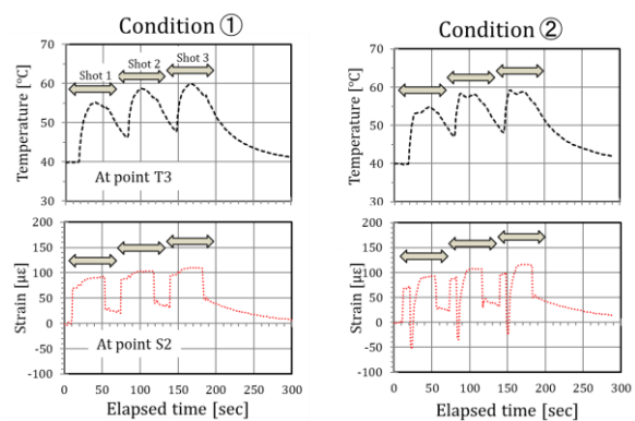
Fig.3 Continuous 3 shots
