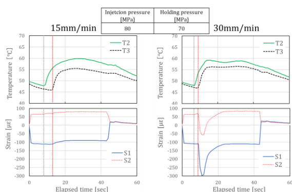
Fig.4 Injection speed
